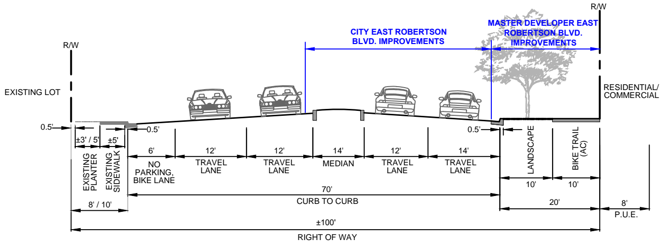
A EAST ROBERTSON BLVD - PHASE 1 SCALE: NTS
