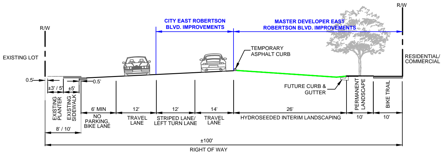
B EAST ROBERTSON BLVD - PHASE 2 & 3 SCALE: NTS
